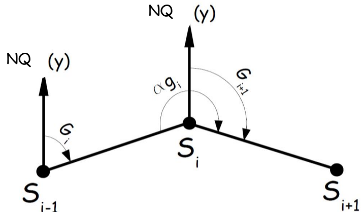
Figure 3.14: Transmission de gisement
